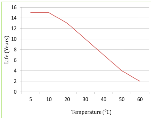
FLOAT SERVICE LIFE CURVE GRAPH
