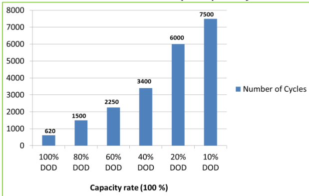
CYCLE LIFE GRAPH (25°C/77°F)
