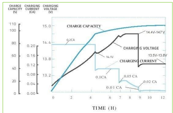
CHARGE CHARACTERISTIC 25°C (77°F)
