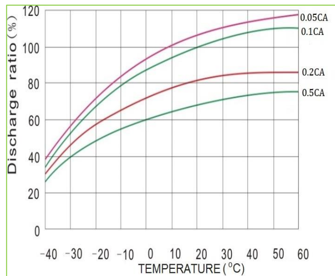
TEMPERATURE AND DISCHARGE CAPACITY
