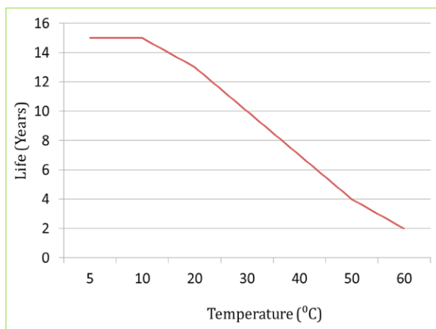
FLOAT SERVICE LIFE CURVE GRAPH
