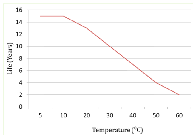
FLOAT SERVICE LIFE CURVE GRAPH
