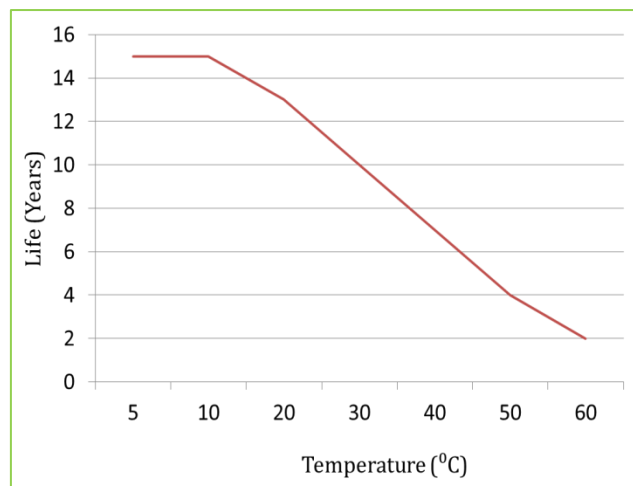
FLOAT SERVICE LIFE CURVE GRAPH
