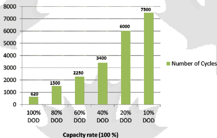
Cycle life graph (25°C/77°F) 12V
